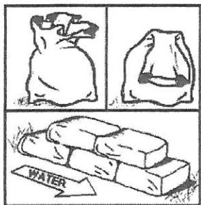
Sandbag placement.
