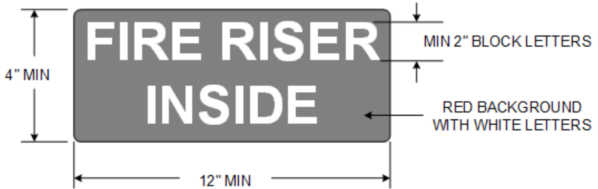
DIAGRAM F-3.3: FIRE RISER SIGN
