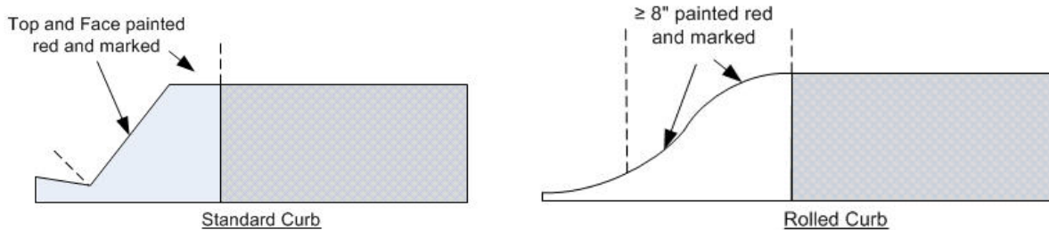
DIAGRAM A-2.2: CURB PAINTING DETAIL
