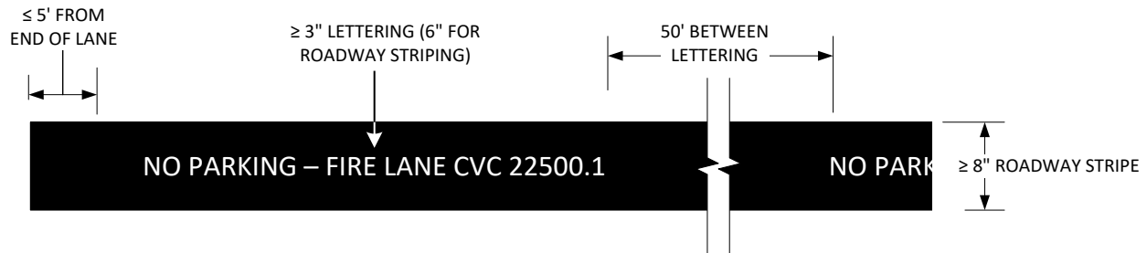
DIAGRAM A-2.3: ROADWAY STRIPING DETAIL
