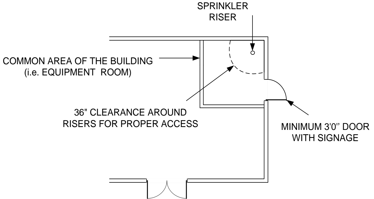
DIAGRAM F-3.1: ACCESS TO SPRINKLER RISERS
