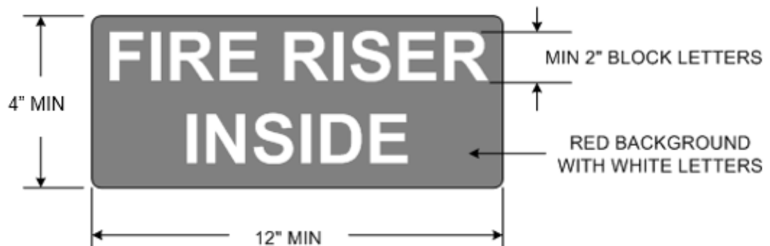
DIAGRAM F-1.4: DETAIL OF "FIRE RISER INSIDE" SIGN (6" X 12")
