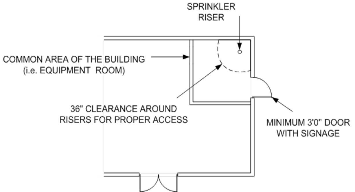
DIAGRAM F-1.2: EXTERIOR ACCESS TO SPRINKLER RISERS
