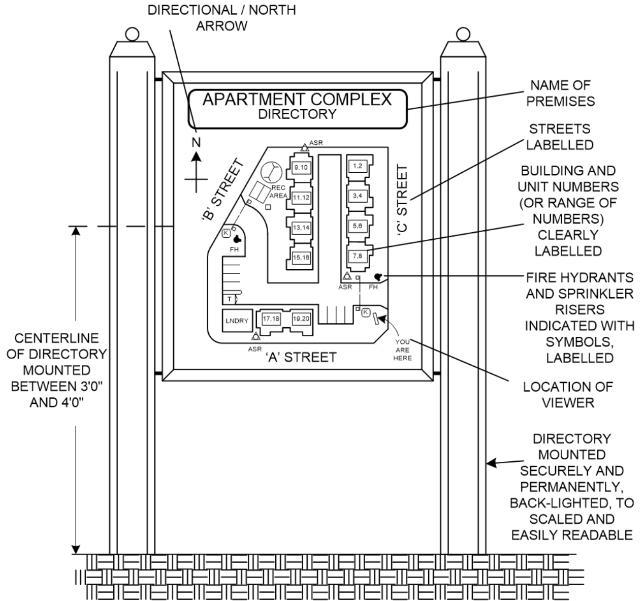
DIAGRAM B-1.1: ILLUMINATED DIRECTORY DETAIL
