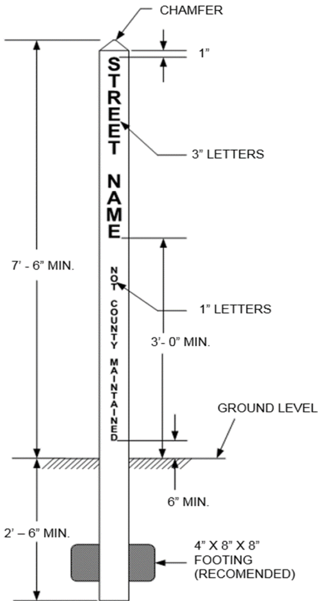
DIAGRAM B-1.2: STREET SIGN POST
